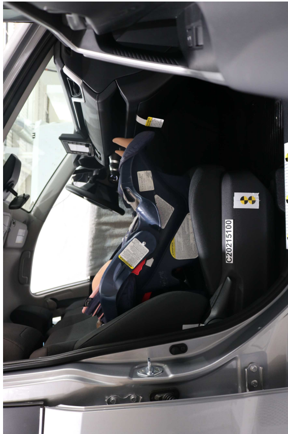
Graco Snuggly W/Out Base, Unbelted, Rear Facing, Rearward Seat Track
