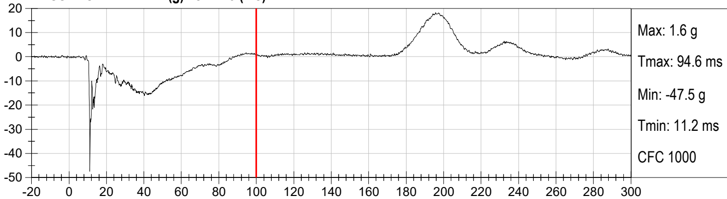
PASSENGER HEAD Y (g) vs Time (ms)
