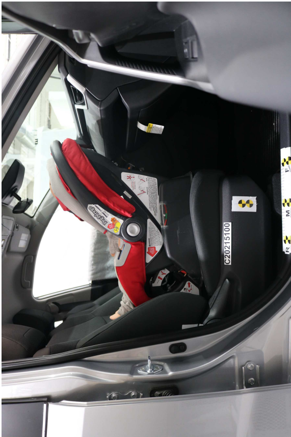
Peg Perego Viaggio WBBase, Unbelted, Rear Facing, Middle Seat Track
