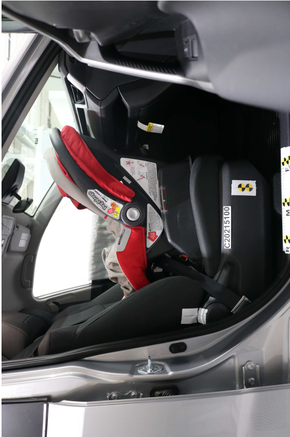
Peg Perego Viaggio WBBase, Belted, Rear Facing, Forward Seat Track
