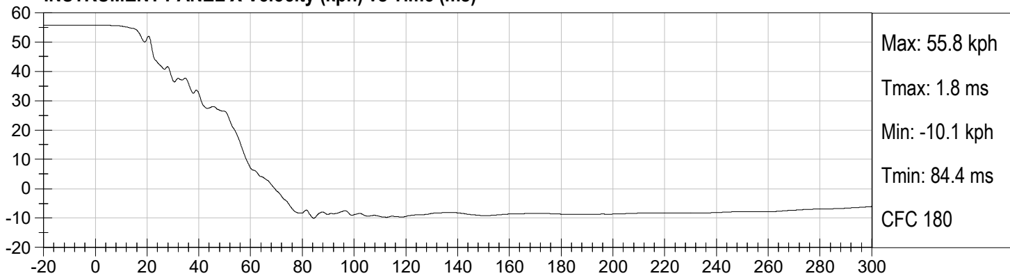
TRUNK Z (g) vs Time (ms)
