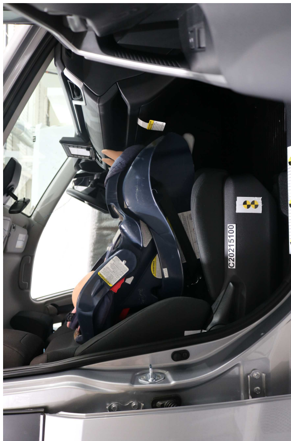
Graco Snugride WBBase, Unbelted, Rear Facing, Rearward Seat Track
