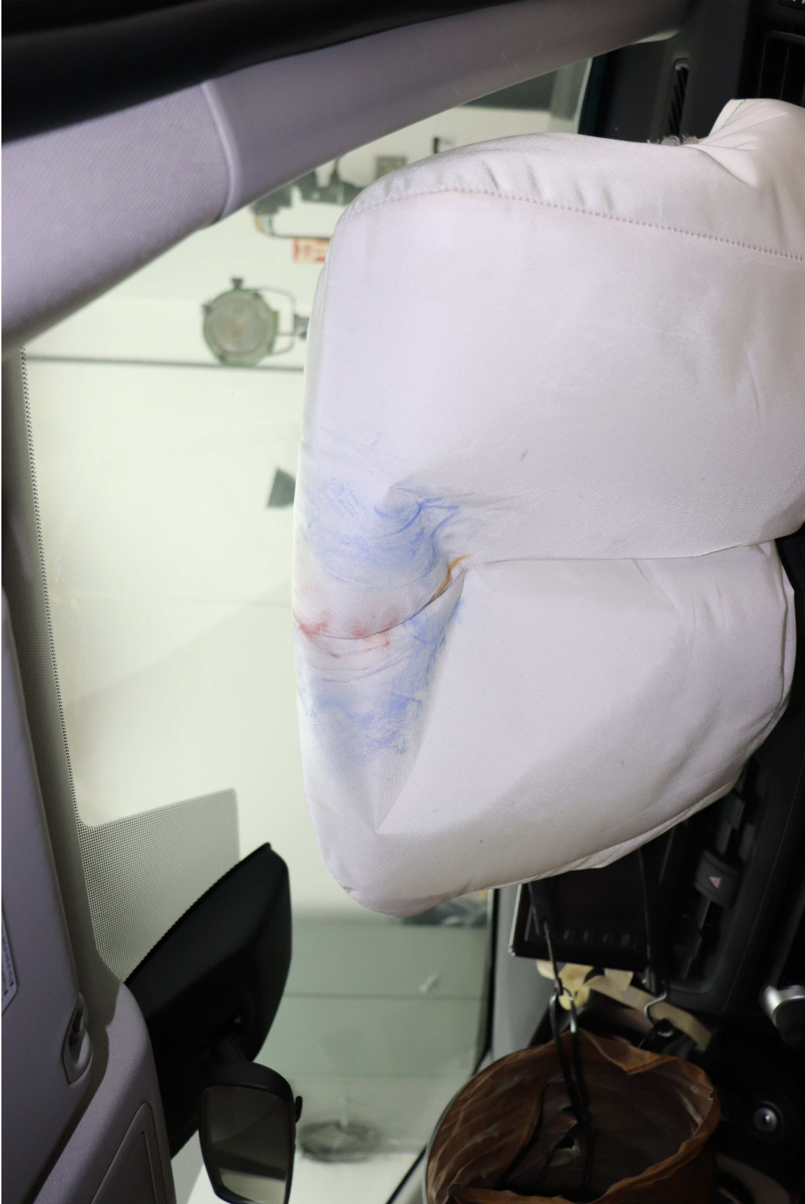
Photo No. 19 - Post-Test 3YO P1 Passenger Dummy Airbag Right Side View
