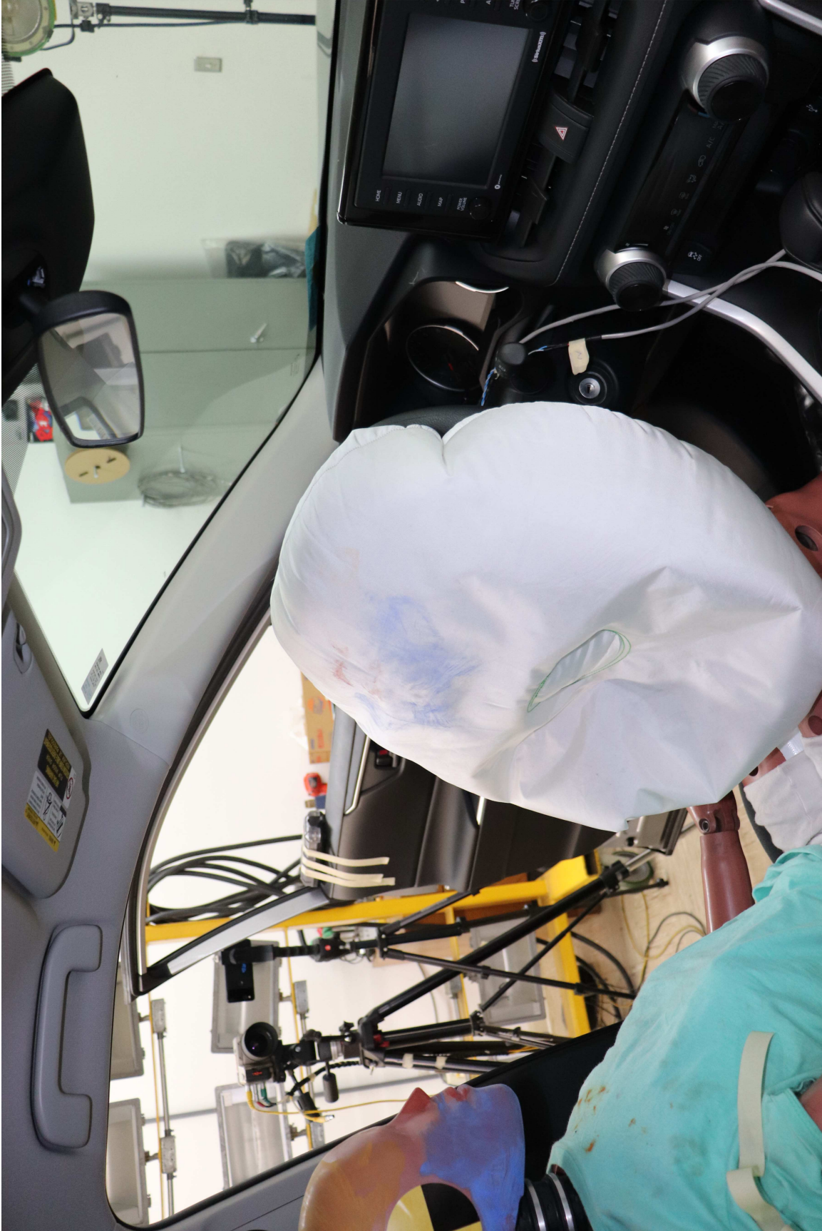
Photo No. 6 - Post-Test 5th Fem. P1 Driver Dummy Airbag Right Side View
