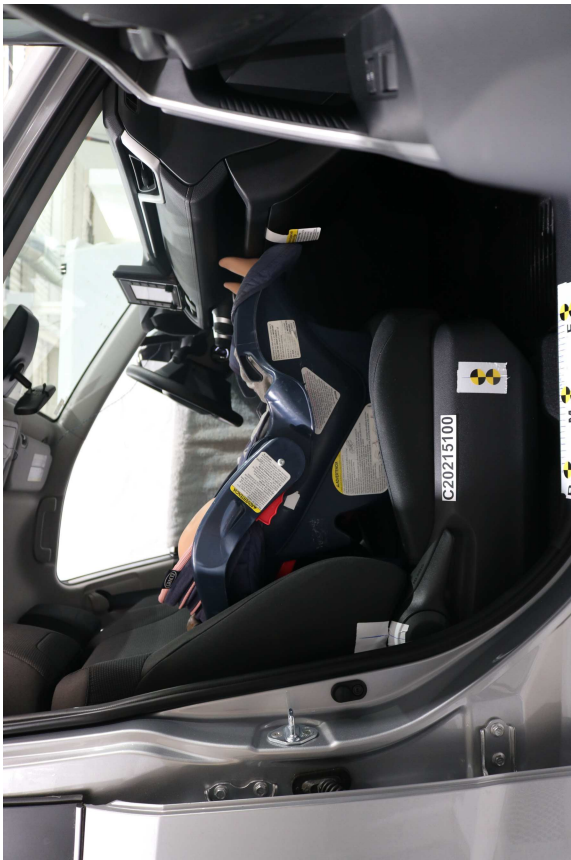
Graco Snuggly W/Out Base, Unbelted, Forward Facing, Forward Seat Track
