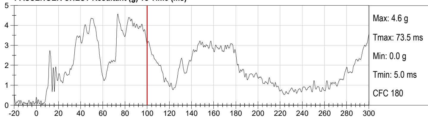
PASSENGER CHEST Resultant (g) vs Time (ms)
