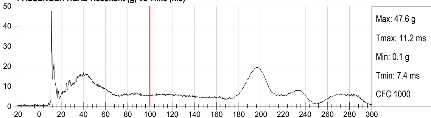
PASSENGER HEAD Resultant (g) vs Time (ms)
