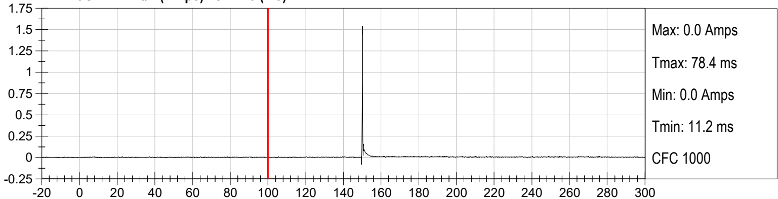
FIRE CURRENT #2 (Amps) vs Time (ms)
